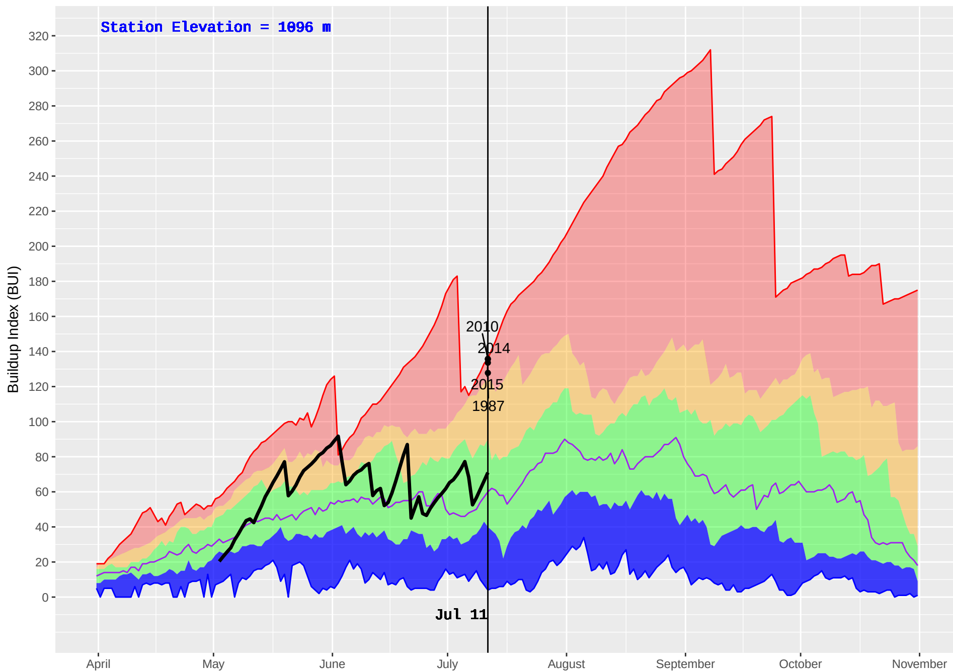
ANAHIM LAKE HUB (213) : Historical (1981–2016) and Current (2018) Noon Buildup Index (BUI)
