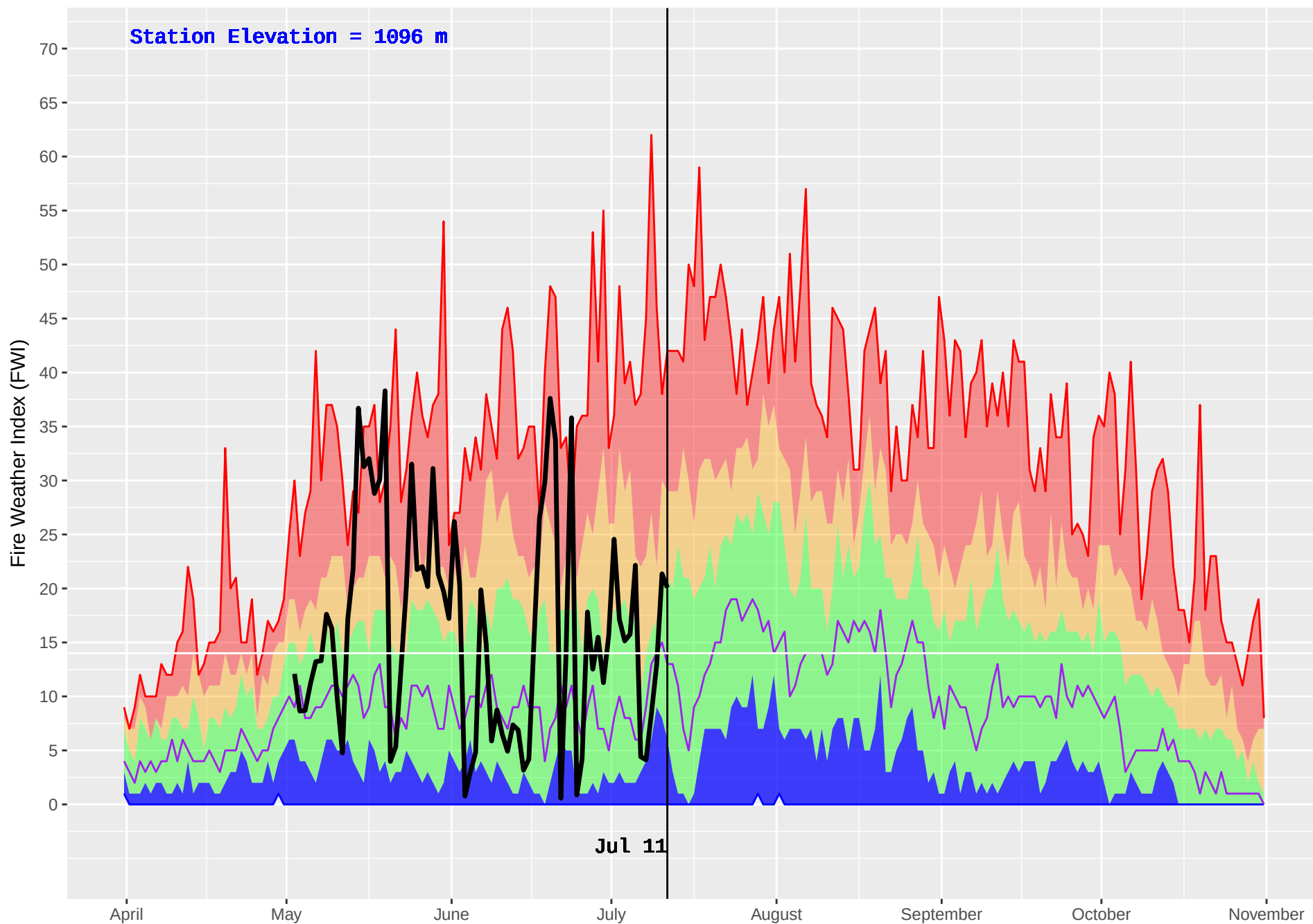
ANAHIM LAKE HUB (213) : Historical (1981–2016) and Current (2018) Noon Fire Weather Index (FWI)
