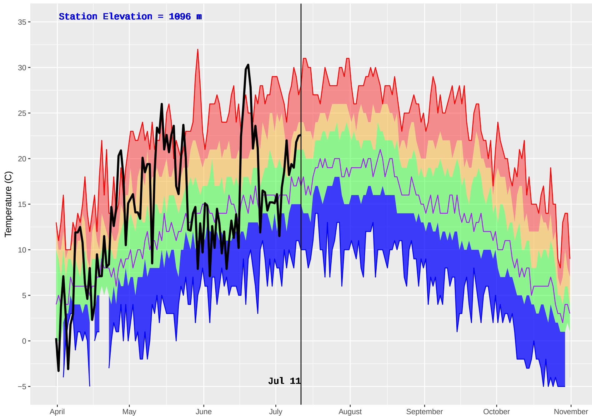
ANAHIM LAKE HUB (213) : Historical (1981–2016) and Current (2018) Noon Temperature
